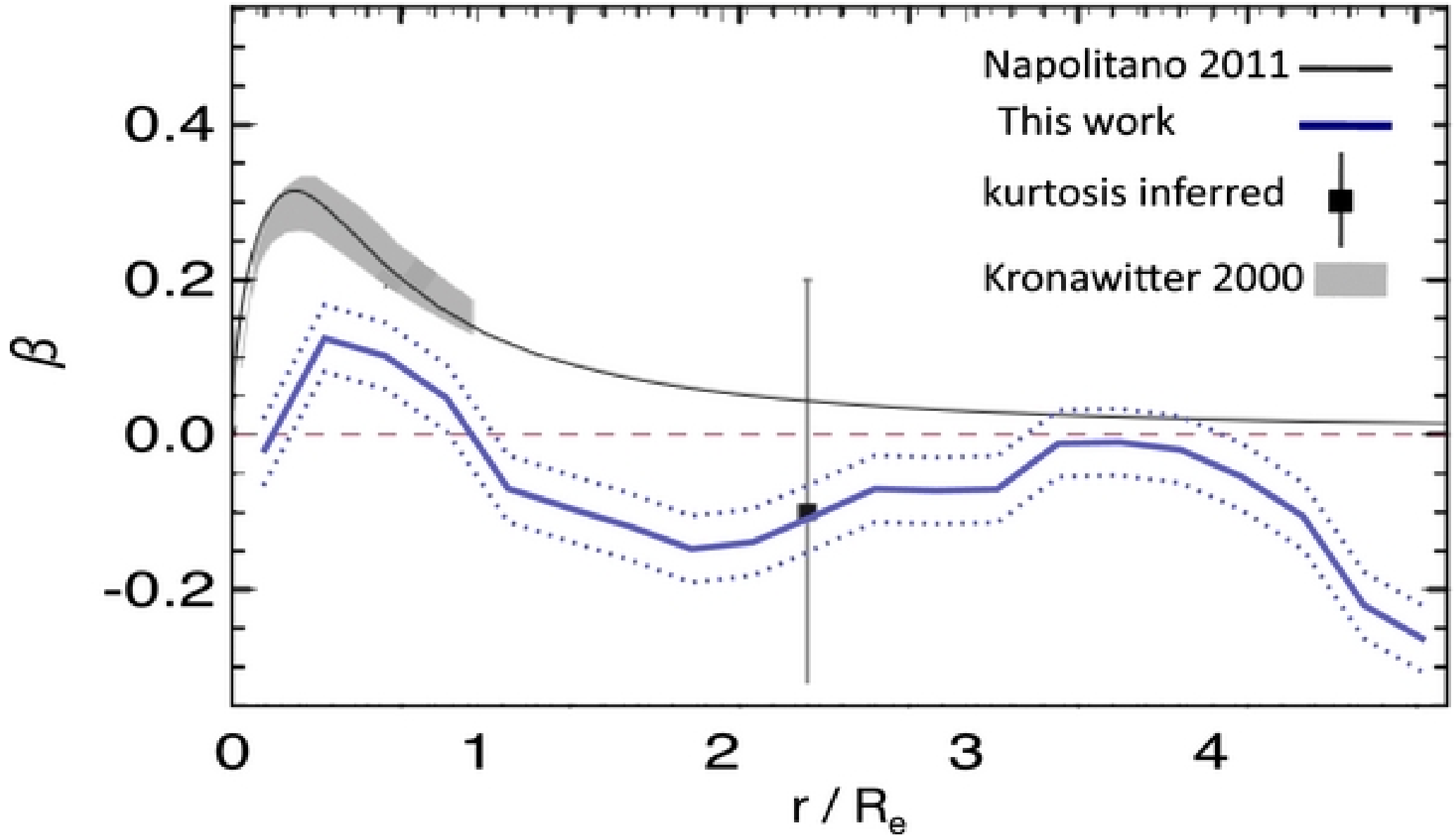
Figure 16. from The Next Generation Virgo Cluster Survey. V. Modeling the Dynamics of M87 with the Made-to-measure Method Zhu et al. 2014 ApJ 792 59 doi:10.1088/0004-637X/792/1/59 https://dx.doi.org/10.1088/0004-637X/792/1/59 © 2014. The American Astronomical Society. All rights reserved.
