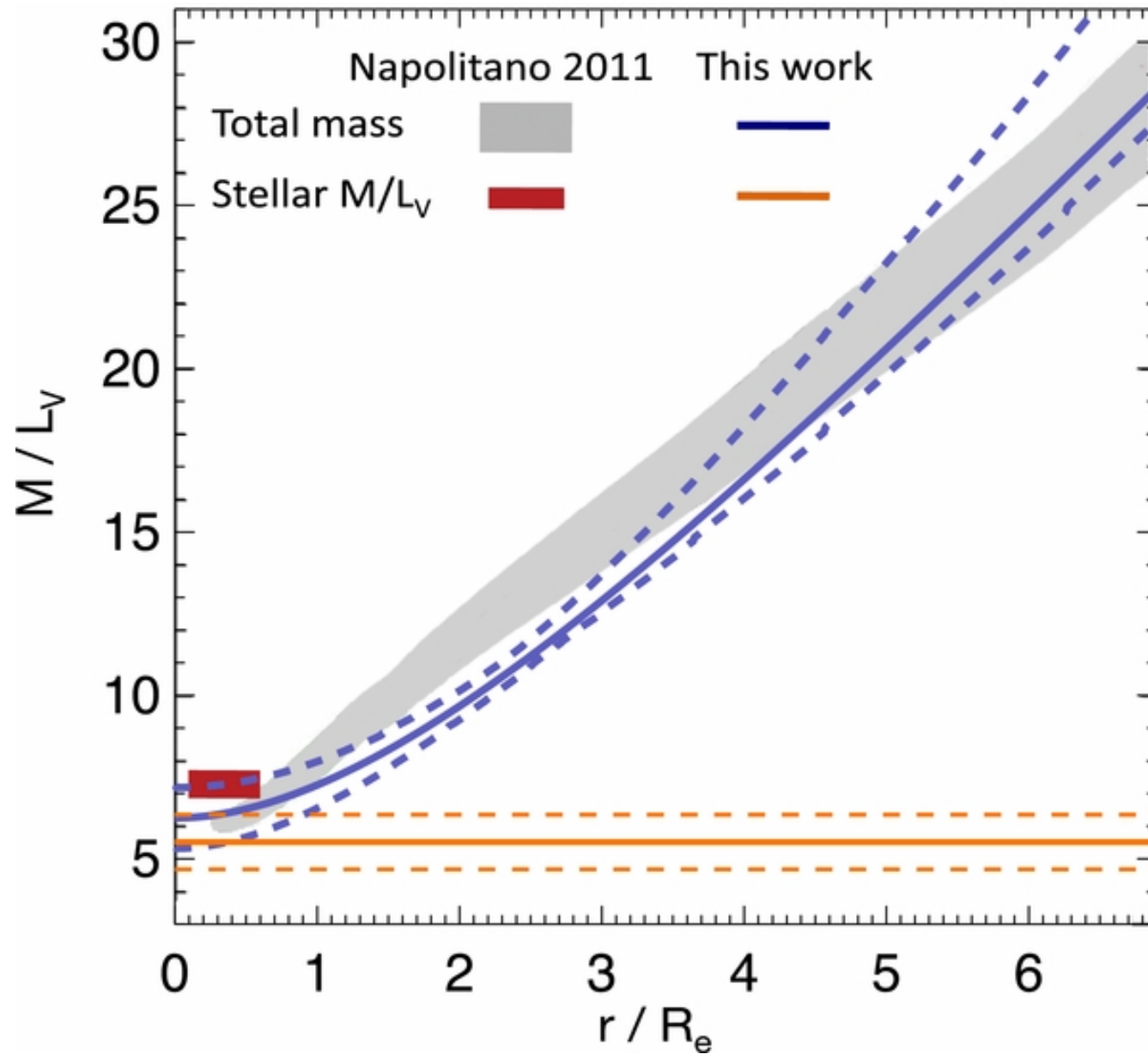
Figure 15. from The Next Generation Virgo Cluster Survey. V. Modeling the Dynamics of M87 with the Made-to-measure Method Zhu et al. 2014 ApJ 792 59 doi:10.1088/0004-637X/792/1/59 https://dx.doi.org/10.1088/0004-637X/792/1/59 © 2014. The American Astronomical Society. All rights reserved.
