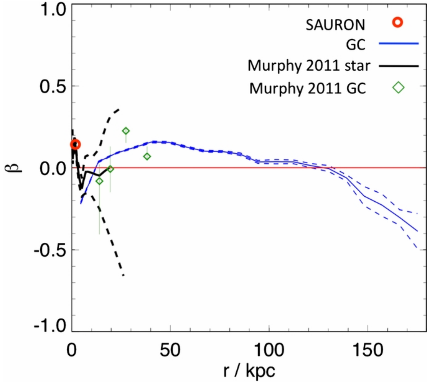
Figure 12. from The Next Generation Virgo Cluster Survey. V. Modeling the Dynamics of M87 with the Made-to-measure Method Zhu et al. 2014 ApJ 792 59 doi:10.1088/0004-637X/792/1/59 https://dx.doi.org/10.1088/0004-637X/792/1/59 © 2014. The American Astronomical Society. All rights reserved.
