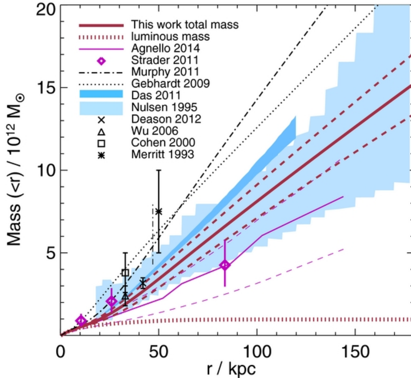
Figure 11. from The Next Generation Virgo Cluster Survey. V. Modeling the Dynamics of M87 with the Made-to-measure Method Zhu et al. 2014 ApJ 792 59 doi:10.1088/0004-637X/792/1/59 https://dx.doi.org/10.1088/0004-637X/792/1/59 © 2014. The American Astronomical Society. All rights reserved.
