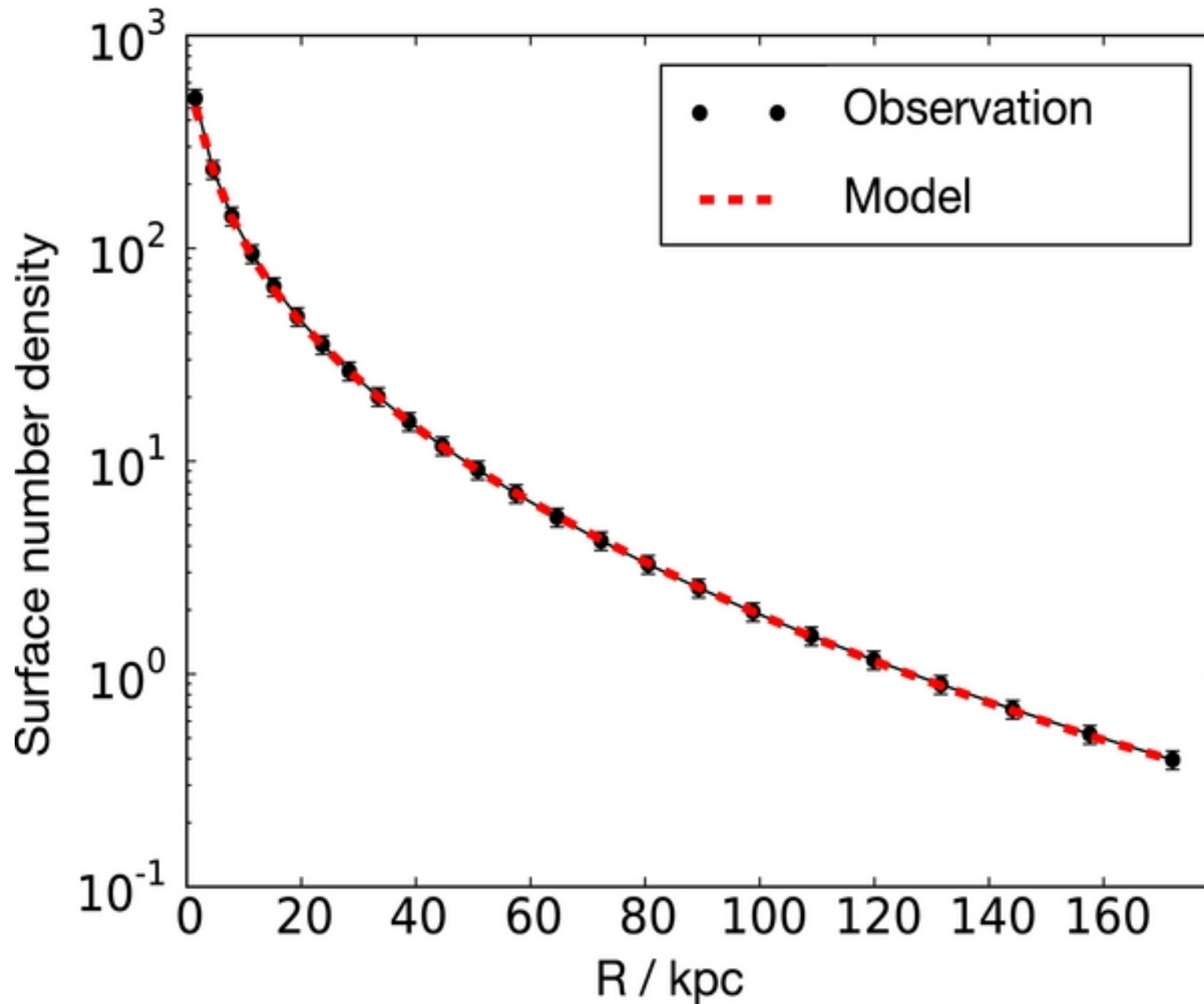
Figure 10. from The Next Generation Virgo Cluster Survey. V. Modeling the Dynamics of M87 with the Made-to-measure Method Zhu et al. 2014 ApJ 792 59 doi:10.1088/0004-637X/792/1/59 https://dx.doi.org/10.1088/0004-637X/792/1/59 © 2014. The American Astronomical Society. All rights reserved.
