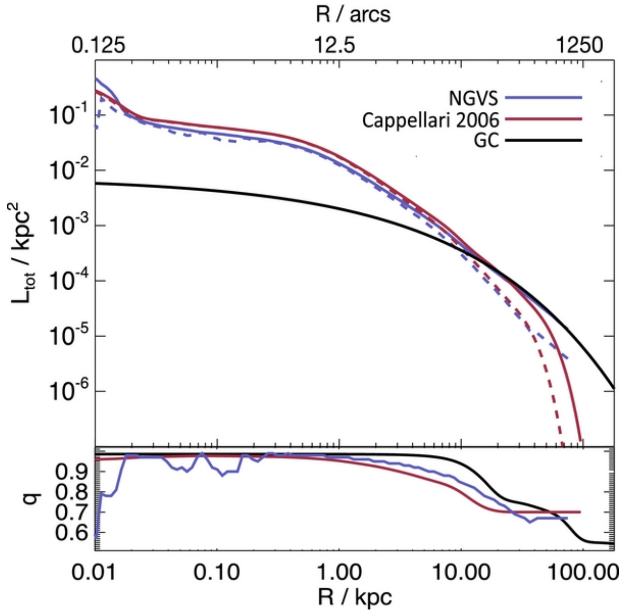
Figure 1. from The Next Generation Virgo Cluster Survey. V. Modeling the Dynamics of M87 with the Made-to-measure Method Zhu et al. 2014 ApJ 792 59 doi:10.1088/0004-637X/792/1/59 https://dx.doi.org/10.1088/0004-637X/792/1/59 © 2014. The American Astronomical Society. All rights reserved.
