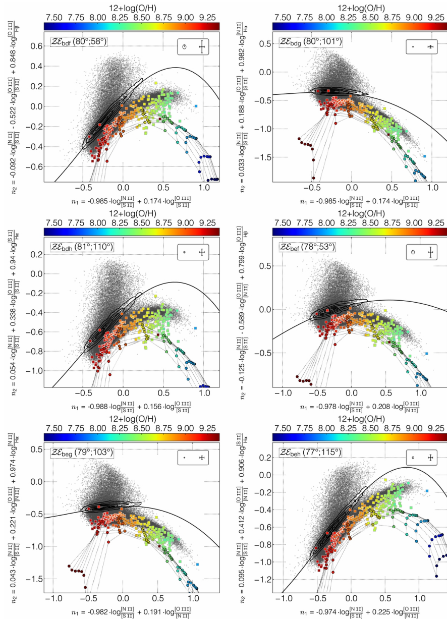
Figure 5. from Galaxy Emission Line Classification Using Three-dimensional Line Ratio Diagrams Vogt et al. 2014 ApJ 793 127 doi:10.1088/0004-637X/793/2/127 https://dx.doi.org/10.1088/0004-637X/793/2/127 © 2014. The American Astronomical Society. All rights reserved.
