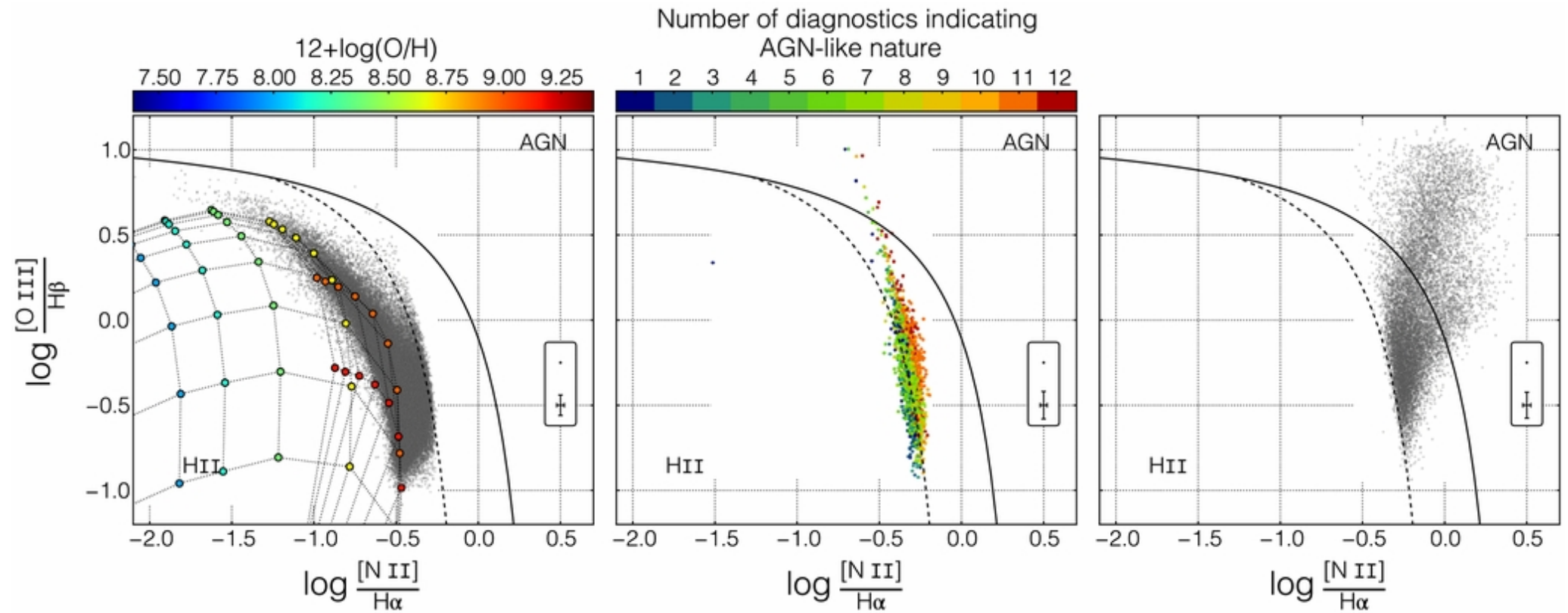
Figure 10. from Galaxy Emission Line Classification Using Three-dimensional Line Ratio Diagrams Vogt et al. 2014 ApJ 793 127 doi:10.1088/0004-637X/793/2/127 https://dx.doi.org/10.1088/0004-637X/793/2/127 © 2014. The American Astronomical Society. All rights reserved.
