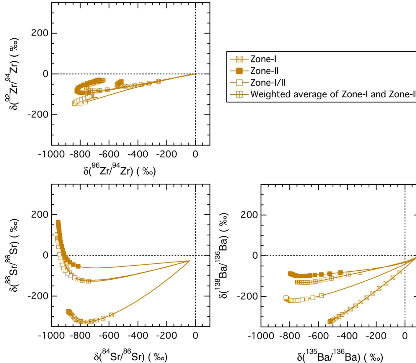
Figure 5. from The ^{13}\text{C} -Pocket Structure in AGB Models: Constraints from Zirconium Isotope Abundances in Single Mainstream SiC Grains Liu et al. 2014 ApJ 788 163 doi:10.1088/0004-637X/788/2/163 https://dx.doi.org/10.1088/0004-637X/788/2/163 © 2014. The American Astronomical Society. All rights reserved.
