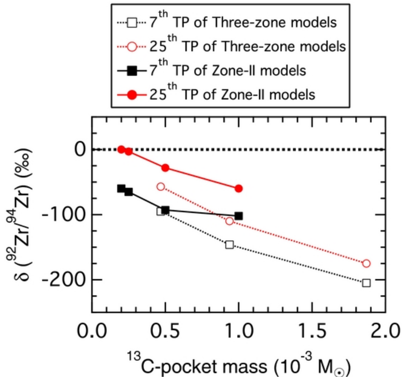
Figure 4. from The ^{13}\text{C} -Pocket Structure in AGB Models: Constraints from Zirconium Isotope Abundances in Single Mainstream SiC Grains Liu et al. 2014 ApJ 788 163 doi:10.1088/0004-637X/788/2/163 https://dx.doi.org/10.1088/0004-637X/788/2/163 © 2014. The American Astronomical Society. All rights reserved.
