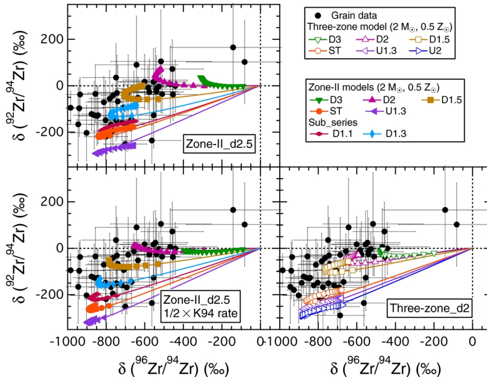
Figure 3. from The ^{13}\text{C} -Pocket Structure in AGB Models: Constraints from Zirconium Isotope Abundances in Single Mainstream SiC Grains Liu et al. 2014 ApJ 788 163 doi:10.1088/0004-637X/788/2/163 https://dx.doi.org/10.1088/0004-637X/788/2/163 © 2014. The American Astronomical Society. All rights reserved.
