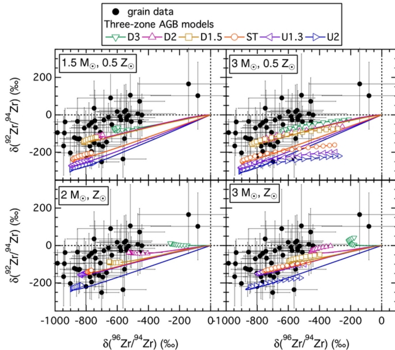
Figure 2. from The ^{13}\text{C} -Pocket Structure in AGB Models: Constraints from Zirconium Isotope Abundances in Single Mainstream SiC Grains Liu et al. 2014 ApJ 788 163 doi:10.1088/0004-637X/788/2/163 https://dx.doi.org/10.1088/0004-637X/788/2/163 © 2014. The American Astronomical Society. All rights reserved.
