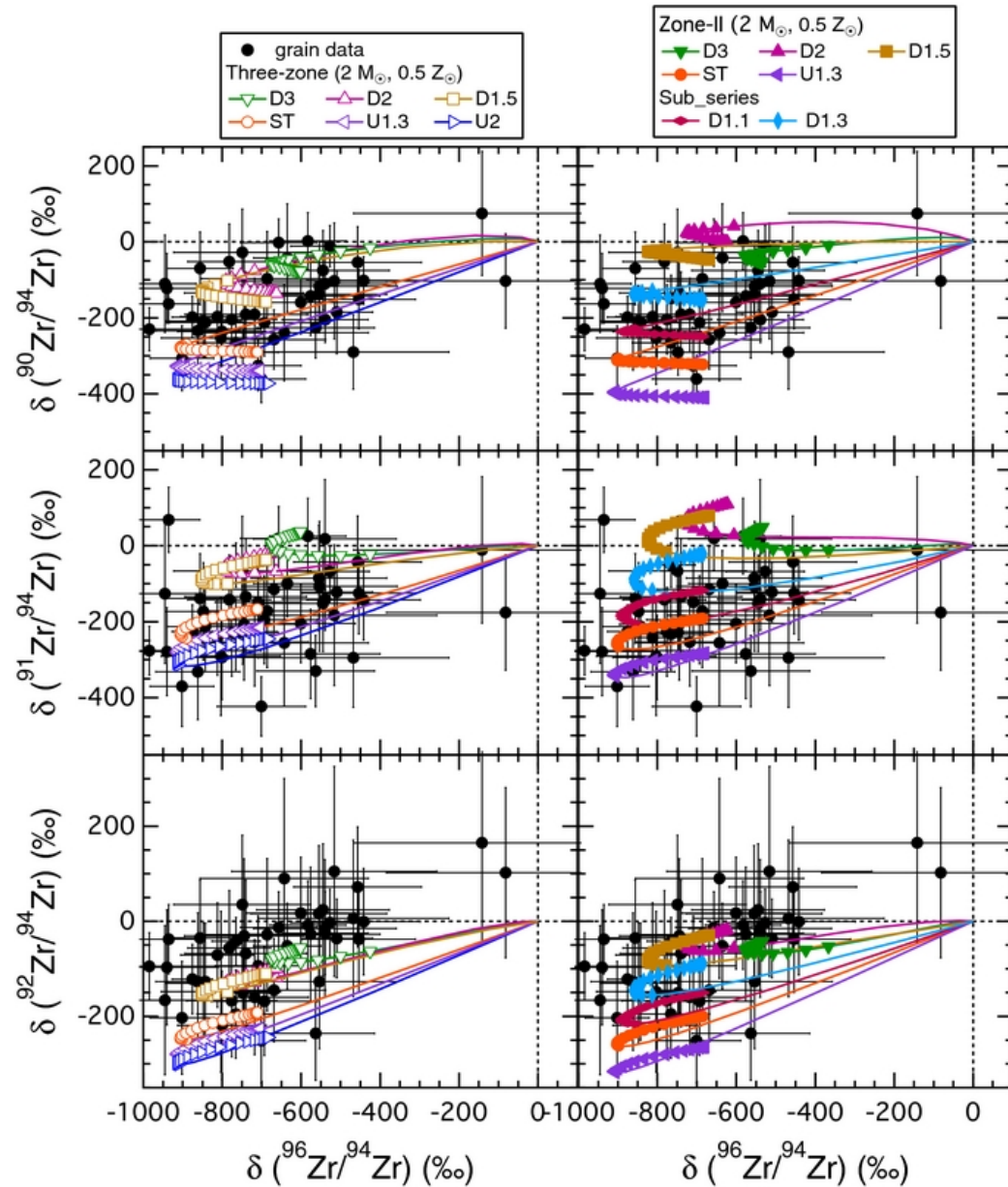
Figure 1. from The ^{13}\text{C} -Pocket Structure in AGB Models: Constraints from Zirconium Isotope Abundances in Single Mainstream SiC Grains Liu et al. 2014 ApJ 788 163 doi:10.1088/0004-637X/788/2/163 https://dx.doi.org/10.1088/0004-637X/788/2/163 © 2014. The American Astronomical Society. All rights reserved.
