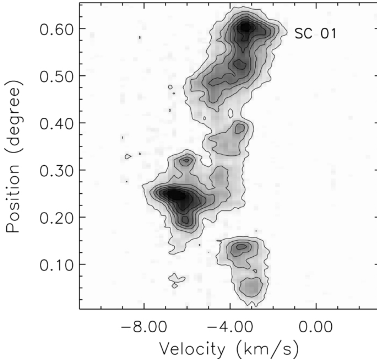
Figure 9. from Molecular Environment of the Supernova Remnant IC 443: Discovery of the Molecular Shells Surrounding the Remnant Su et al. 2014 ApJ 788 122 doi:10.1088/0004-637X/788/2/122 https://dx.doi.org/10.1088/0004-637X/788/2/122 © 2014. The American Astronomical Society. All rights reserved.
