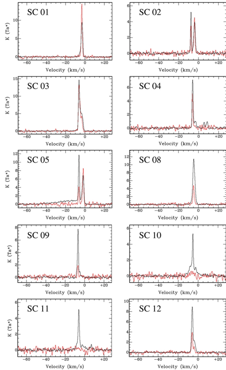
Figure 5. from Molecular Environment of the Supernova Remnant IC 443: Discovery of the Molecular Shells Surrounding the Remnant Su et al. 2014 ApJ 788 122 doi:10.1088/0004-637X/788/2/122 https://dx.doi.org/10.1088/0004-637X/788/2/122
