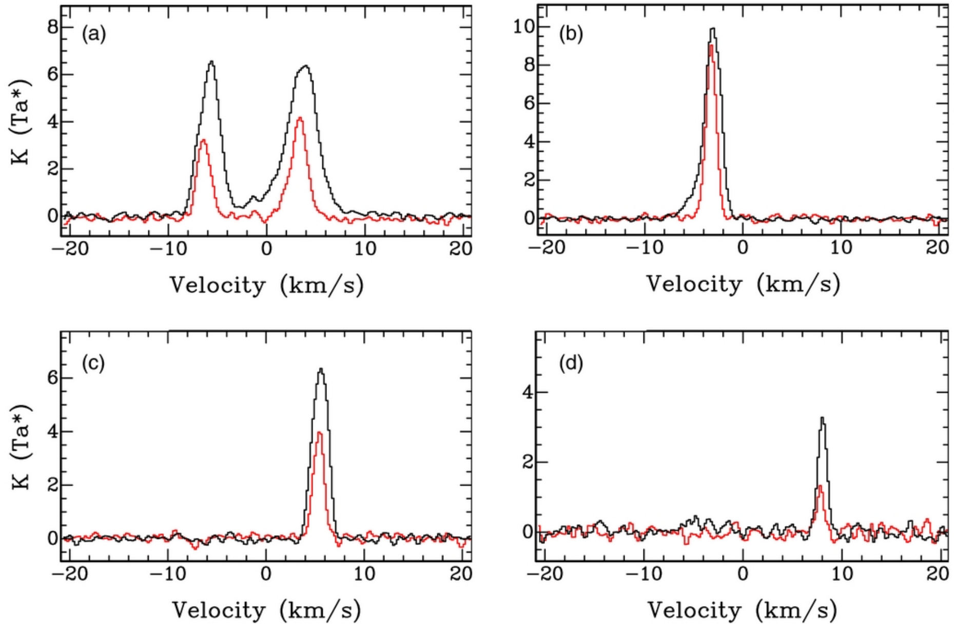
Figure 4. from Molecular Environment of the Supernova Remnant IC 443: Discovery of the Molecular Shells Surrounding the Remnant Su et al. 2014 ApJ 788 122 doi:10.1088/0004-637X/788/2/122 https://dx.doi.org/10.1088/0004-637X/788/2/122 © 2014. The American Astronomical Society. All rights reserved.
