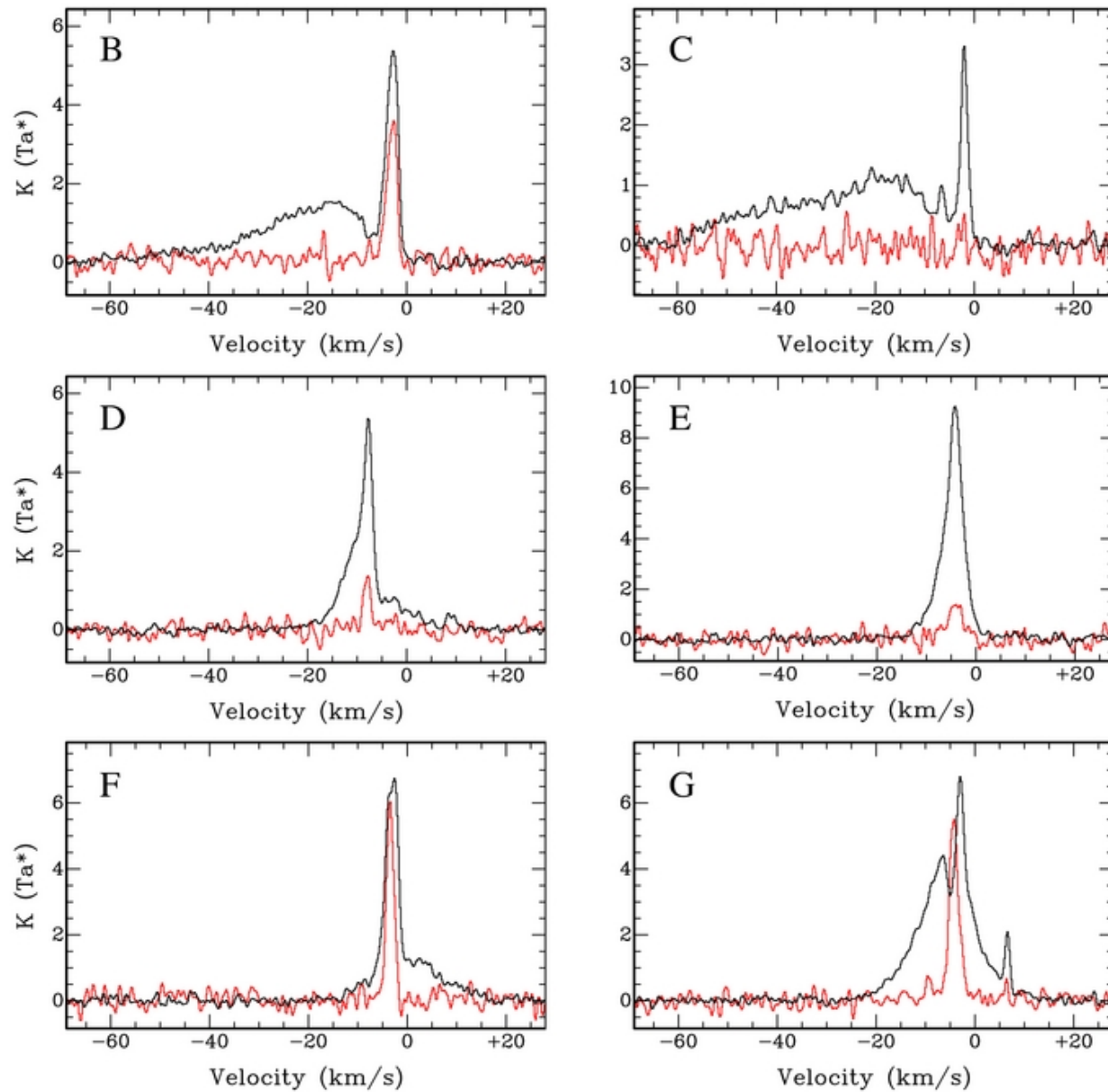
Figure 2. from Molecular Environment of the Supernova Remnant IC 443: Discovery of the Molecular Shells Surrounding the Remnant Su et al. 2014 ApJ 788 122 doi:10.1088/0004-637X/788/2/122 https://dx.doi.org/10.1088/0004-637X/788/2/122 © 2014. The American Astronomical Society. All rights reserved.
