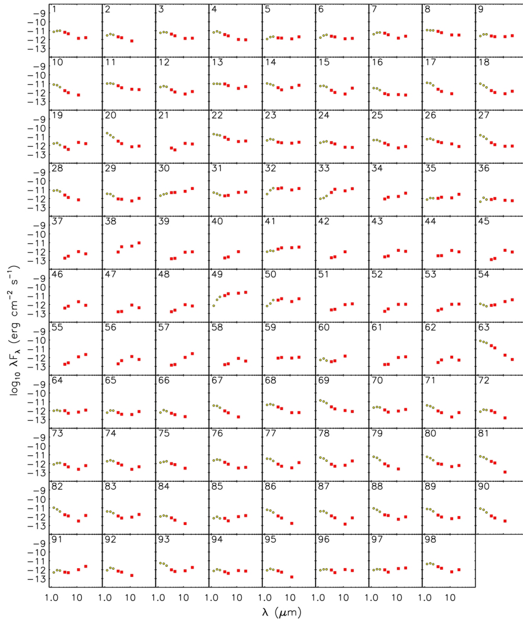
Figure 14. from Molecular Environment of the Supernova Remnant IC 443: Discovery of the Molecular Shells Surrounding the Remnant Su et al. 2014 ApJ 788 122 doi:10.1088/0004-637X/788/2/122 https://dx.doi.org/10.1088/0004-637X/788/2/122 © 2014. The American Astronomical Society. All rights reserved.
