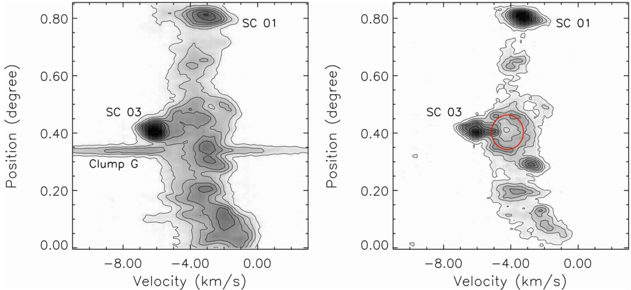
Figure 13. from Molecular Environment of the Supernova Remnant IC 443: Discovery of the Molecular Shells Surrounding the Remnant Su et al. 2014 ApJ 788 122 doi:10.1088/0004-637X/788/2/122 https://dx.doi.org/10.1088/0004-637X/788/2/122 © 2014. The American Astronomical Society. All rights reserved.
