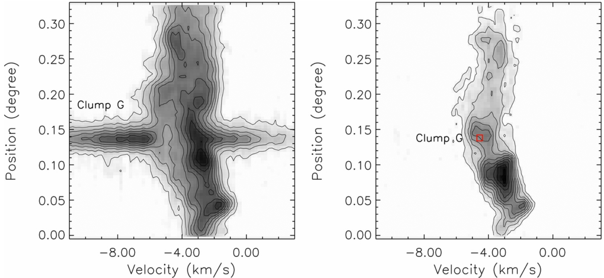
Figure 12. from Molecular Environment of the Supernova Remnant IC 443: Discovery of the Molecular Shells Surrounding the Remnant Su et al. 2014 ApJ 788 122 doi:10.1088/0004-637X/788/2/122 https://dx.doi.org/10.1088/0004-637X/788/2/122 © 2014. The American Astronomical Society. All rights reserved.
