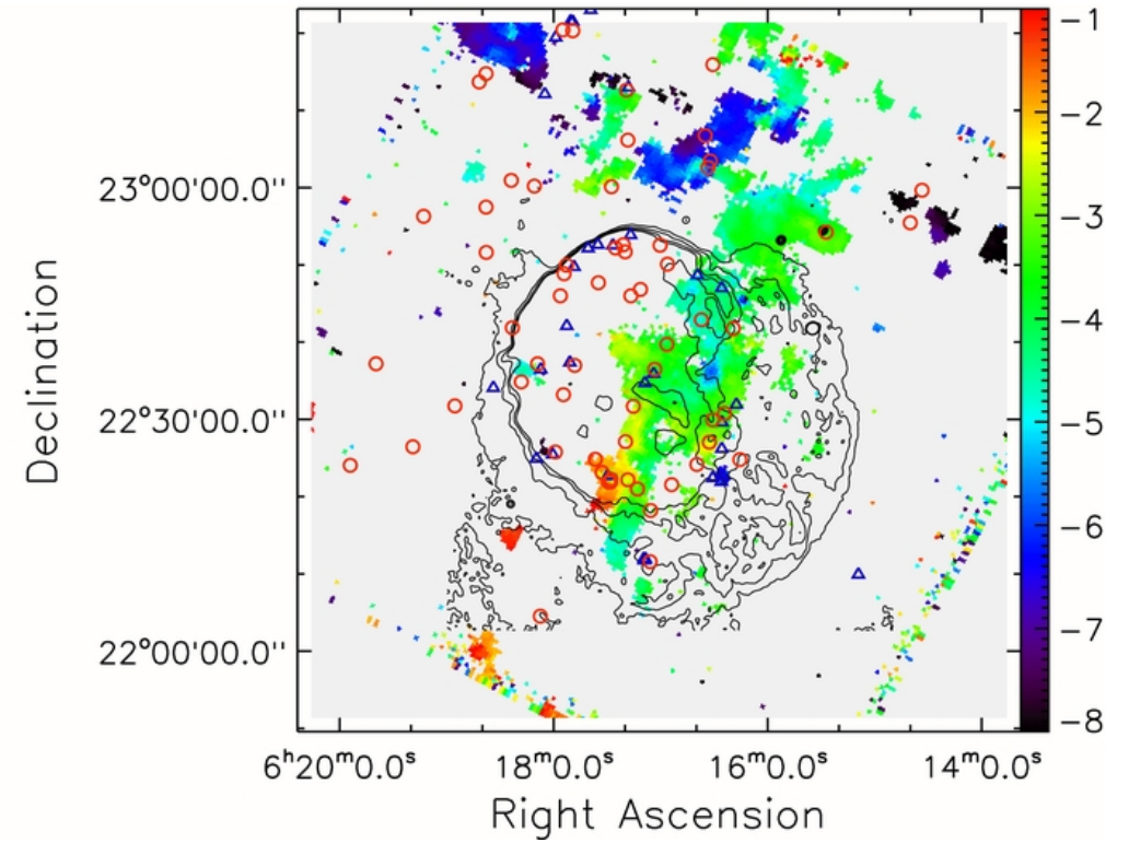
Figure 11. from Molecular Environment of the Supernova Remnant IC 443: Discovery of the Molecular Shells Surrounding the Remnant Su et al. 2014 ApJ 788 122 doi:10.1088/0004-637X/788/2/122 https://dx.doi.org/10.1088/0004-637X/788/2/122 © 2014. The American Astronomical Society. All rights reserved.
