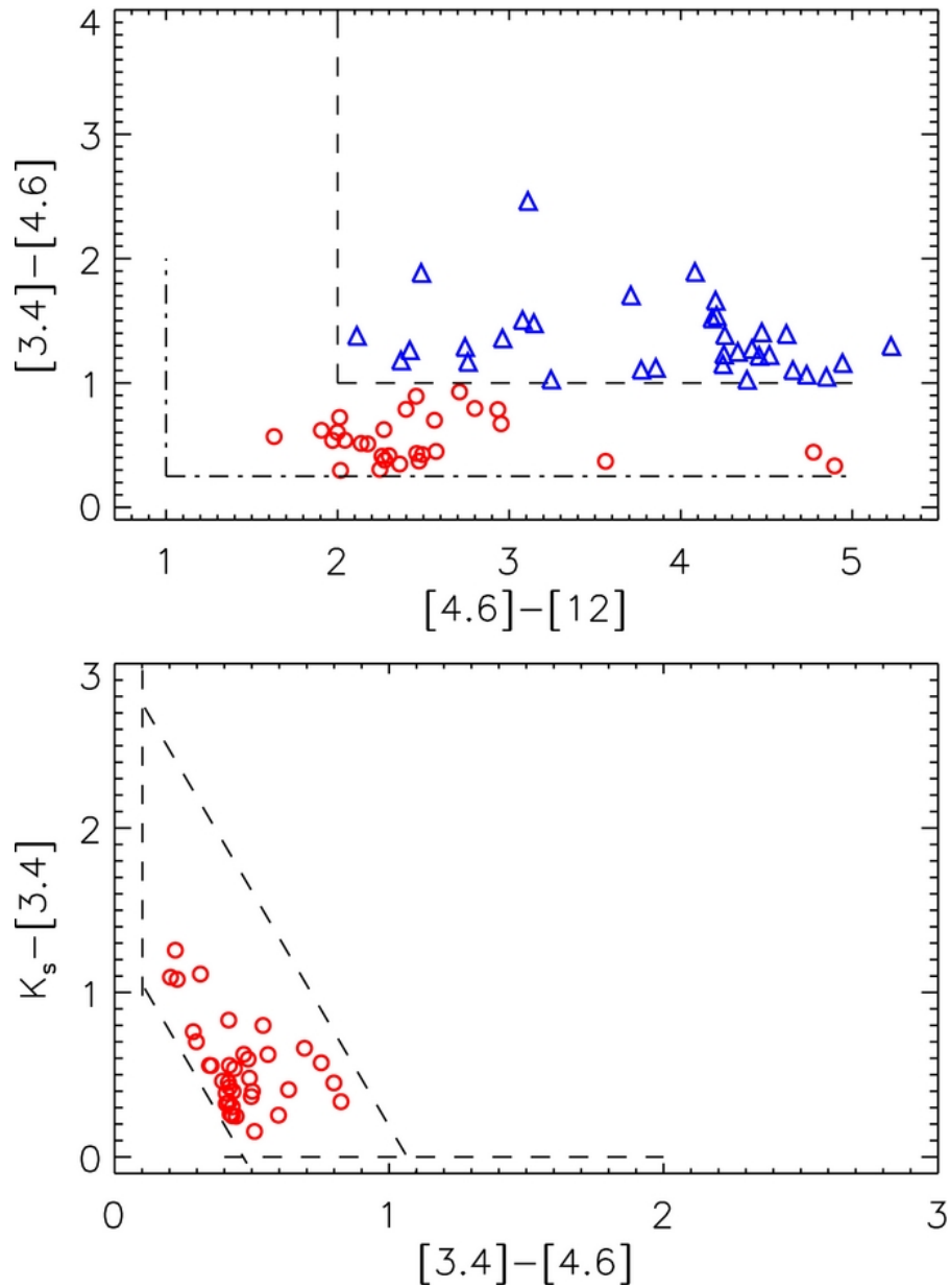
Figure 10. from Molecular Environment of the Supernova Remnant IC 443: Discovery of the Molecular Shells Surrounding the Remnant Su et al. 2014 ApJ 788 122 doi:10.1088/0004-637X/788/2/122 https://dx.doi.org/10.1088/0004-637X/788/2/122
