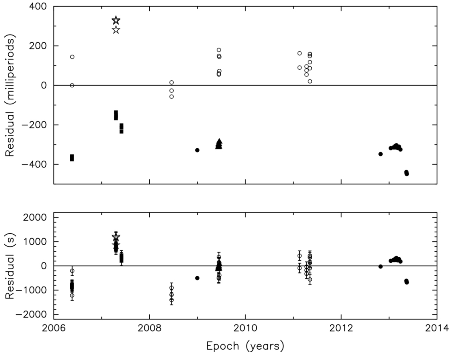
Figure 2. from Timing Analysis of the Periodic Radio and Optical Brightness Variations of the Ultracool Dwarf, TVLM 513-46546 Wolszczan & Route 2014 ApJ 788 23 doi:10.1088/0004-637X/788/1/23 https://dx.doi.org/10.1088/0004-637X/788/1/23 © 2014. The American Astronomical Society. All rights reserved.
