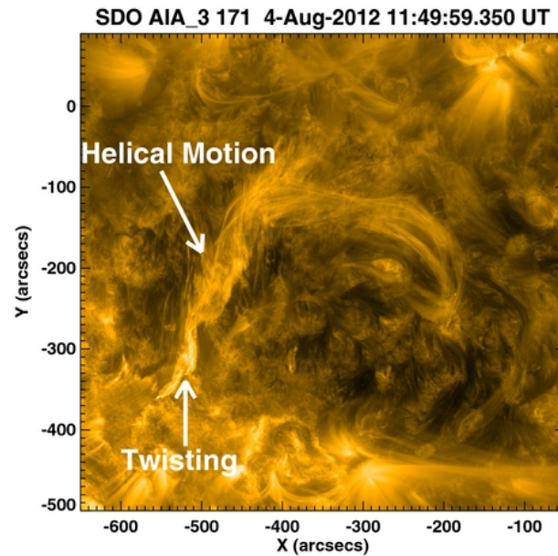
Figure 7. from Fast Magnetic Twister and Plasma Perturbations in a Three-dimensional Coronal Arcade Murawski, Srivastava, & Musielak 2014 ApJ 788 8 doi:10.1088/0004-637X/788/1/8 https://dx.doi.org/10.1088/0004-637X/788/1/8 © 2014. The American Astronomical Society. All rights reserved.
