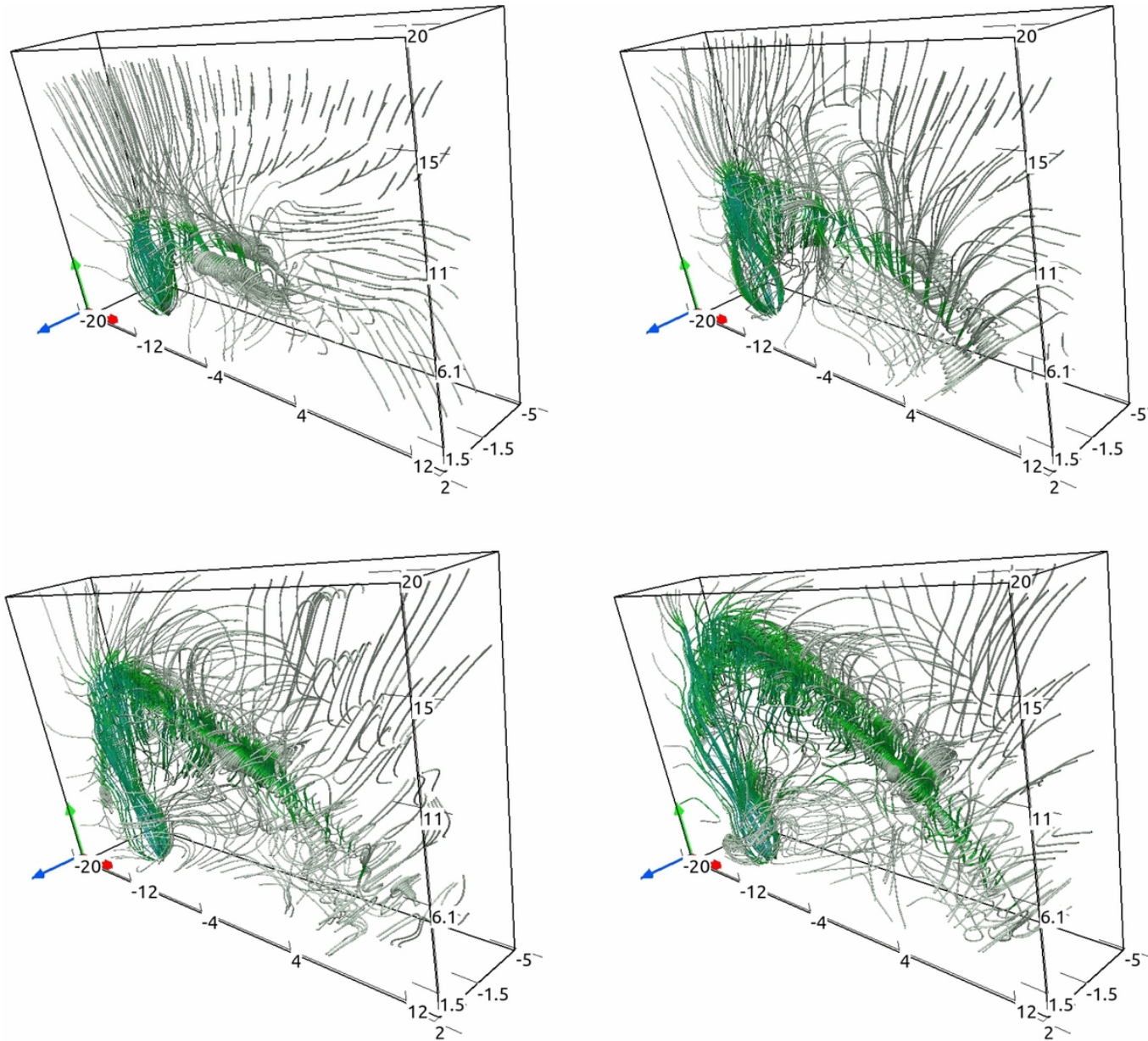
Figure 5. from Fast Magnetic Twister and Plasma Perturbations in a Three-dimensional Coronal Arcade Murawski, Srivastava, & Musielak 2014 ApJ 788 8 doi:10.1088/0004-637X/788/1/8 https://dx.doi.org/10.1088/0004-637X/788/1/8 © 2014. The American Astronomical Society. All rights reserved.
