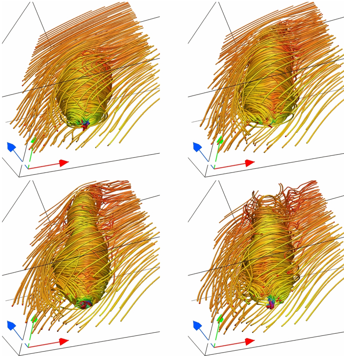
Figure 4. from Fast Magnetic Twister and Plasma Perturbations in a Three-dimensional Coronal Arcade Murawski, Srivastava, & Musielak 2014 ApJ 788 8 doi:10.1088/0004-637X/788/1/8 https://dx.doi.org/10.1088/0004-637X/788/1/8 © 2014. The American Astronomical Society. All rights reserved.
