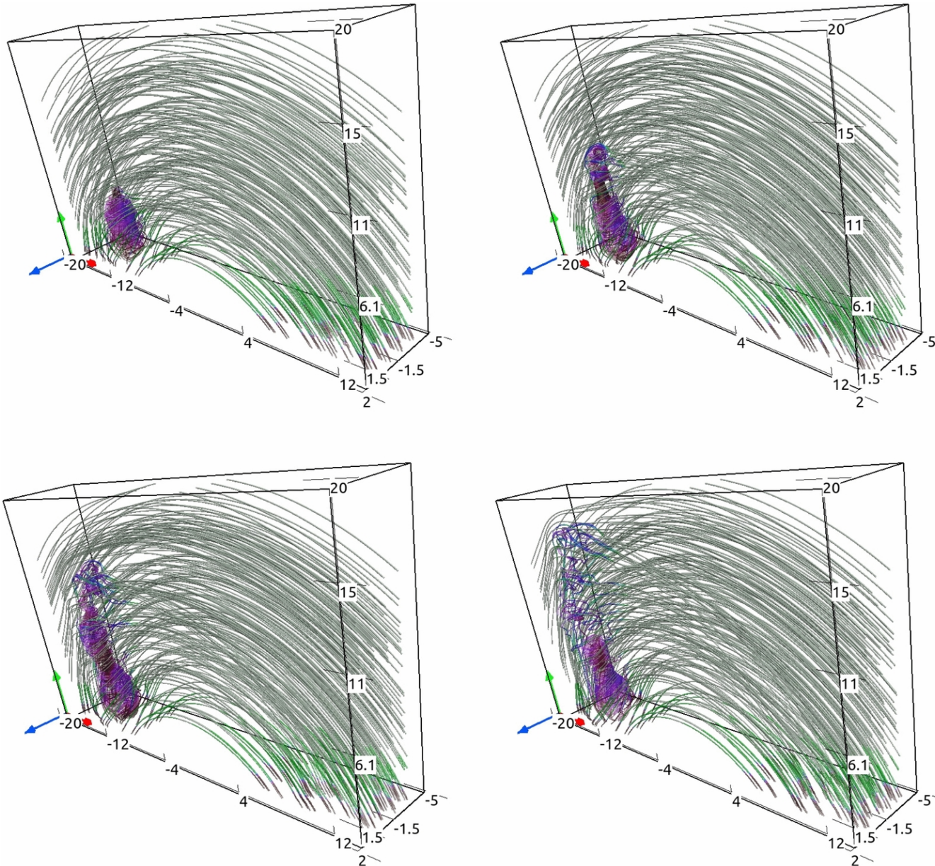
Figure 3. from Fast Magnetic Twister and Plasma Perturbations in a Three-dimensional Coronal Arcade Murawski, Srivastava, & Musielak 2014 ApJ 788 8 doi:10.1088/0004-637X/788/1/8 https://dx.doi.org/10.1088/0004-637X/788/1/8 © 2014. The American Astronomical Society. All rights reserved.
