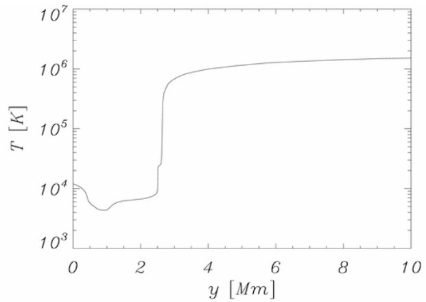
Figure 1. from Fast Magnetic Twister and Plasma Perturbations in a Three-dimensional Coronal Arcade Murawski, Srivastava, & Musielak 2014 ApJ 788 8 doi:10.1088/0004-637X/788/1/8 https://dx.doi.org/10.1088/0004-637X/788/1/8
