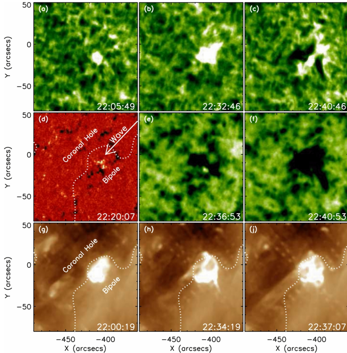
Figure 5. from A Chain of Winking (Oscillating) Filaments Triggered by an Invisible Extreme-ultraviolet Wave Shen et al. 2014 ApJ 786 151 doi:10.1088/0004-637X/786/2/151 https://dx.doi.org/10.1088/0004-637X/786/2/151
