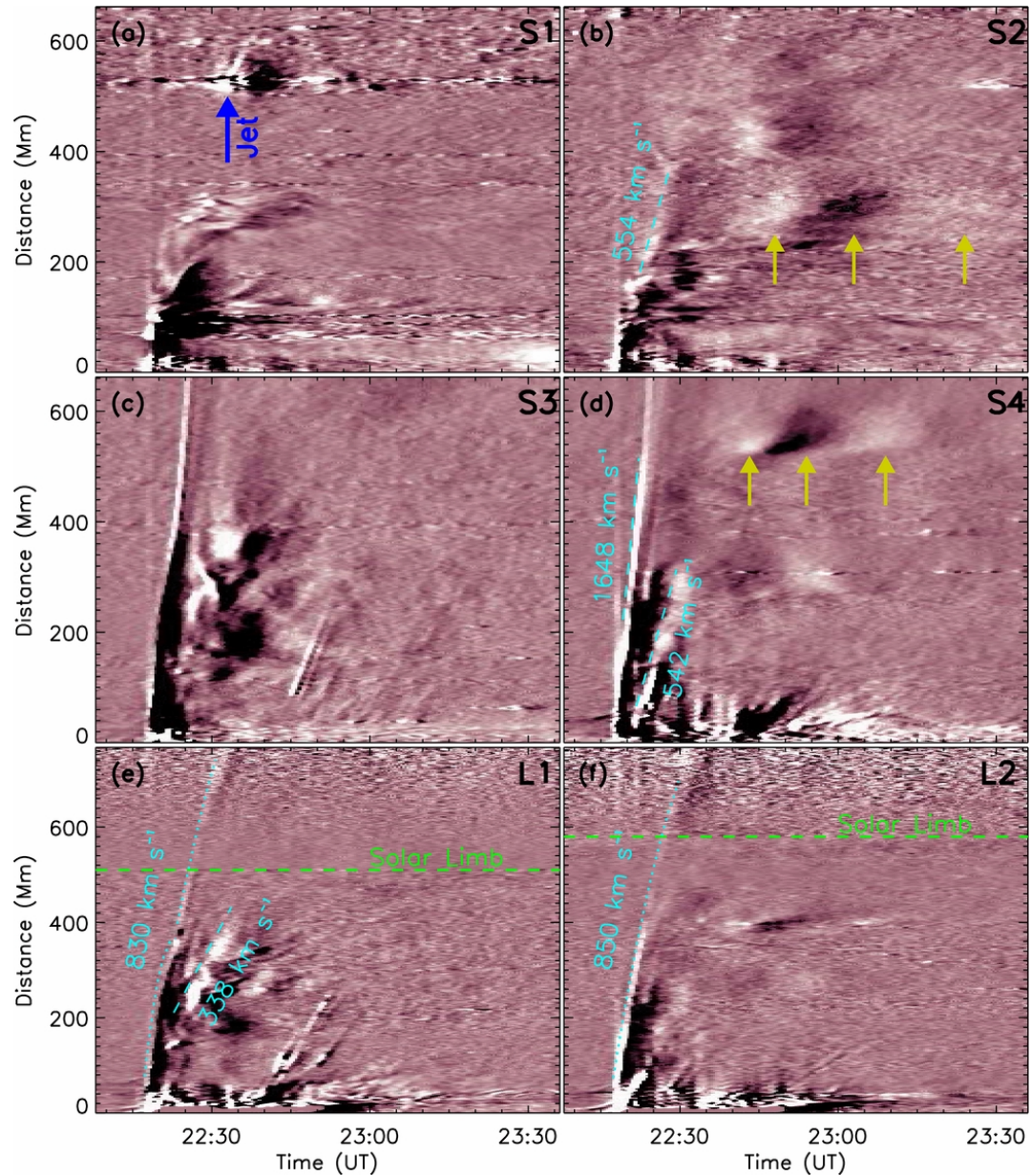
Figure 2. from A Chain of Winking (Oscillating) Filaments Triggered by an Invisible Extreme-ultraviolet Wave Shen et al. 2014 ApJ 786 151 doi:10.1088/0004-637X/786/2/151 https://dx.doi.org/10.1088/0004-637X/786/2/151
