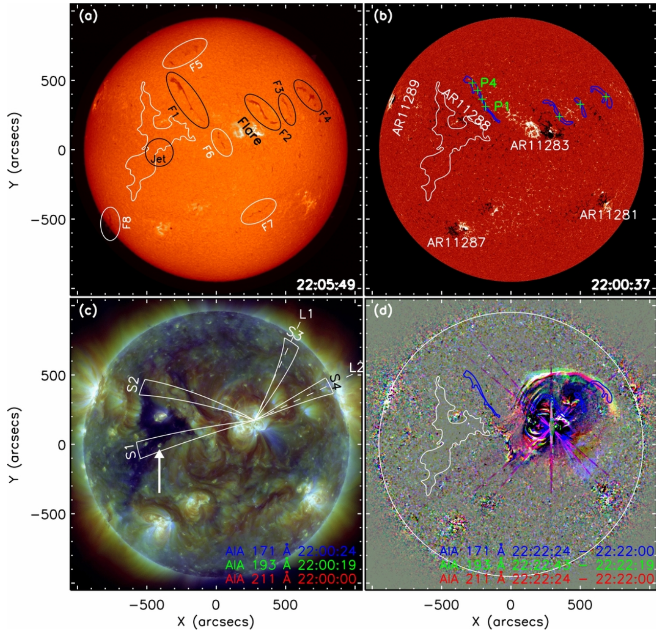
Figure 1. from A Chain of Winking (Oscillating) Filaments Triggered by an Invisible Extreme-ultraviolet Wave Shen et al. 2014 ApJ 786 151 doi:10.1088/0004-637X/786/2/151 https://dx.doi.org/10.1088/0004-637X/786/2/151 © 2014. The American Astronomical Society. All rights reserved.
