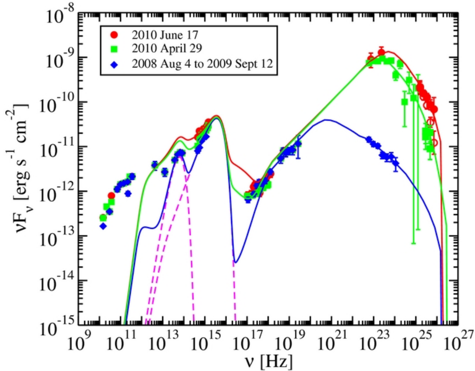
Figure 9. from Multifrequency Studies of the Peculiar Quasar 4C +21.35 during the 2010 Flaring Activity Ackermann et al. 2014 ApJ 786 157 doi:10.1088/0004-637X/786/2/157 https://dx.doi.org/10.1088/0004-637X/786/2/157 © 2014. The American Astronomical Society. All rights reserved.
