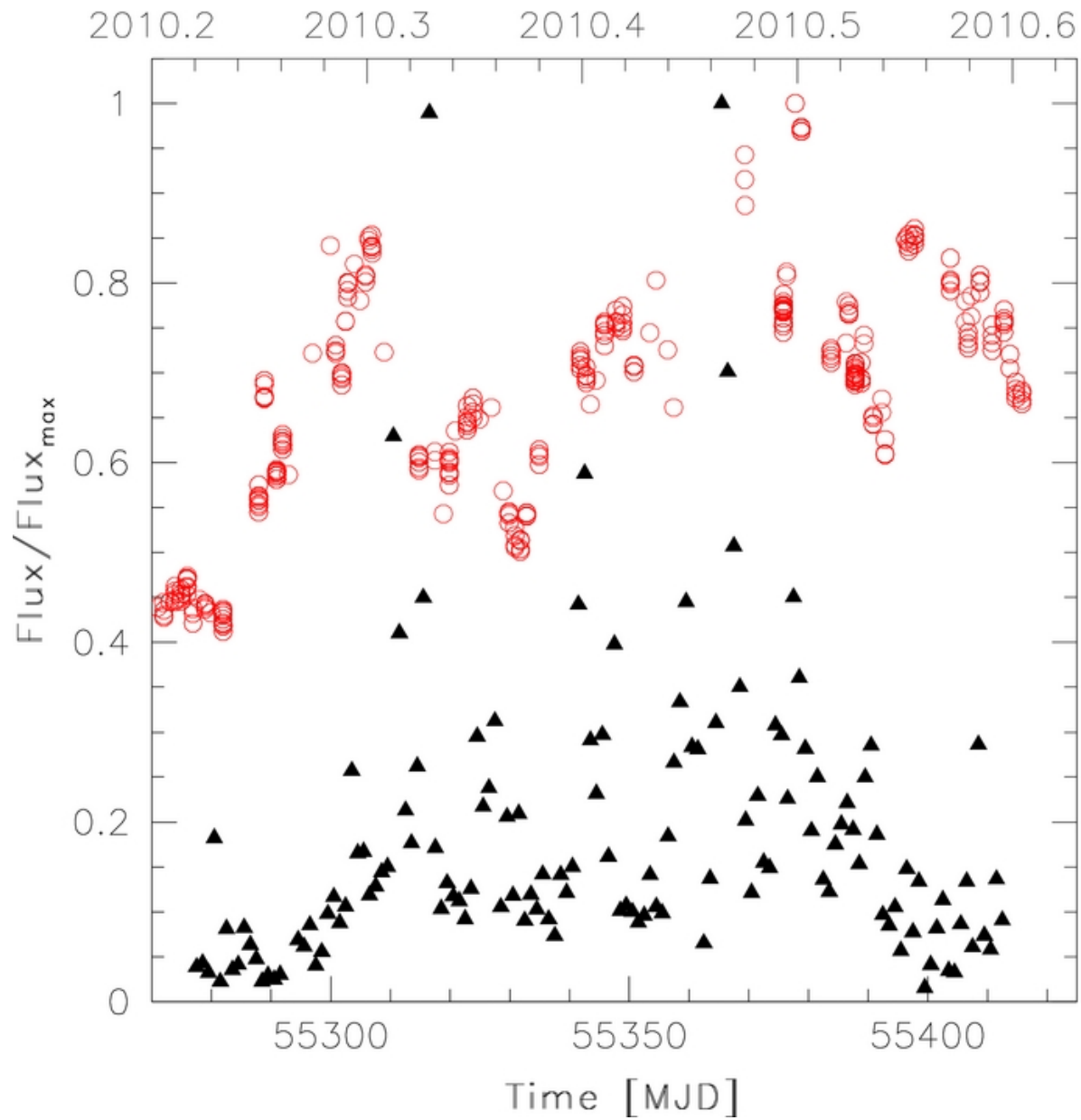
Figure 8. from Multifrequency Studies of the Peculiar Quasar 4C +21.35 during the 2010 Flaring Activity Ackermann et al. 2014 ApJ 786 157 doi:10.1088/0004-637X/786/2/157 https://dx.doi.org/10.1088/0004-637X/786/2/157 © 2014. The American Astronomical Society. All rights reserved.
