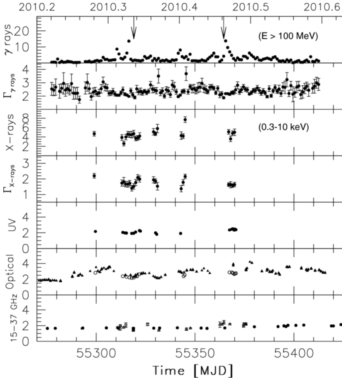
Figure 6. from Multifrequency Studies of the Peculiar Quasar 4C +21.35 during the 2010 Flaring Activity Ackermann et al. 2014 ApJ 786 157 doi:10.1088/0004-637X/786/2/157 https://dx.doi.org/10.1088/0004-637X/786/2/157 © 2014. The American Astronomical Society. All rights reserved.
