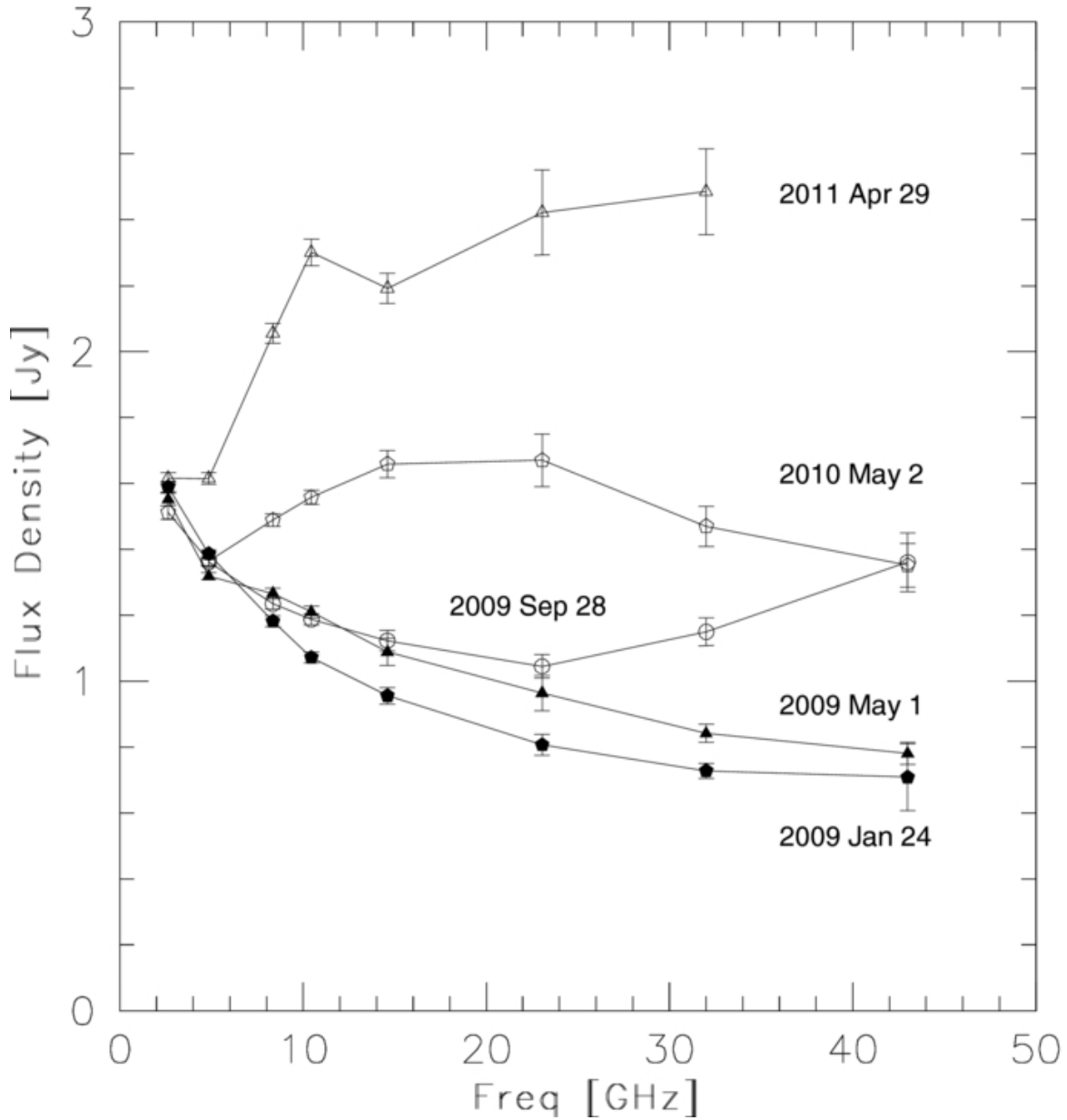
Figure 3. from Multifrequency Studies of the Peculiar Quasar 4C +21.35 during the 2010 Flaring Activity Ackermann et al. 2014 ApJ 786 157 doi:10.1088/0004-637X/786/2/157 https://dx.doi.org/10.1088/0004-637X/786/2/157 © 2014. The American Astronomical Society. All rights reserved.
