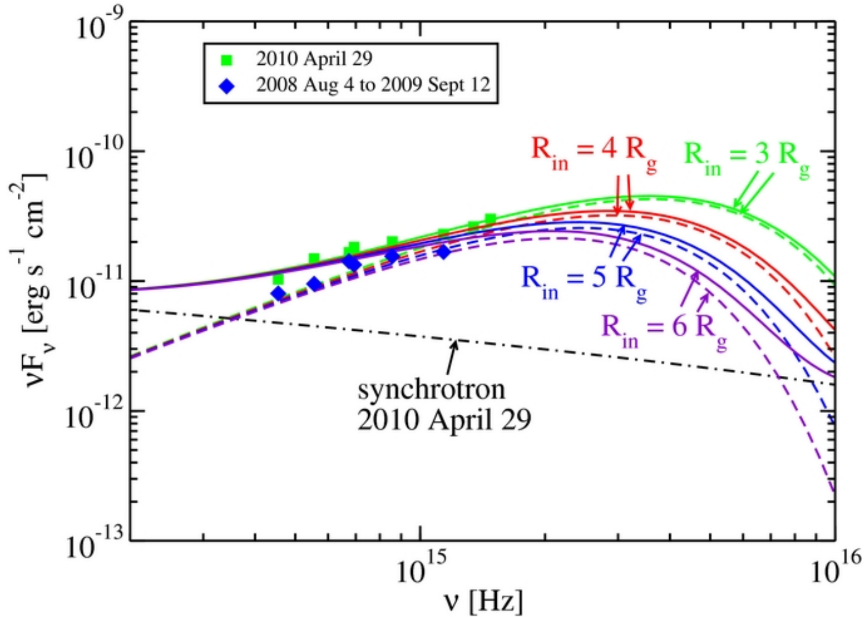
Figure 10. from Multifrequency Studies of the Peculiar Quasar 4C +21.35 during the 2010 Flaring Activity Ackermann et al. 2014 ApJ 786 157 doi:10.1088/0004-637X/786/2/157 https://dx.doi.org/10.1088/0004-637X/786/2/157 © 2014. The American Astronomical Society. All rights reserved.
