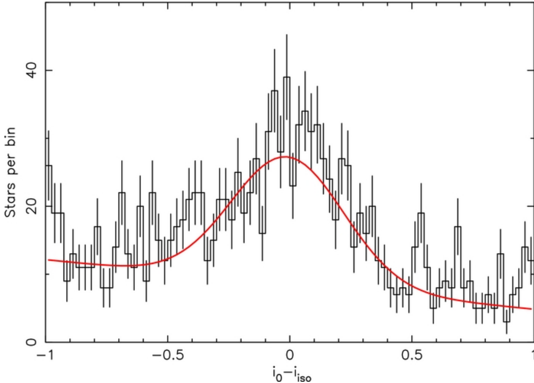
Figure 5. from The PAndAS Field of Streams: Stellar Structures in the Milky Way Halo toward Andromeda and Triangulum Martin et al. 2014 ApJ 787 19 doi:10.1088/0004-637X/787/1/19 https://dx.doi.org/10.1088/0004-637X/787/1/19 © 2014. The American Astronomical Society. All rights reserved.
