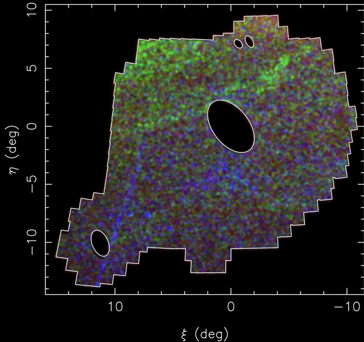
Figure 3. from The PAndAS Field of Streams: Stellar Structures in the Milky Way Halo toward Andromeda and Triangulum Martin et al. 2014 ApJ 787 19 doi:10.1088/0004-637X/787/1/19 https://dx.doi.org/10.1088/0004-637X/787/1/19 © 2014. The American Astronomical Society. All rights reserved.
