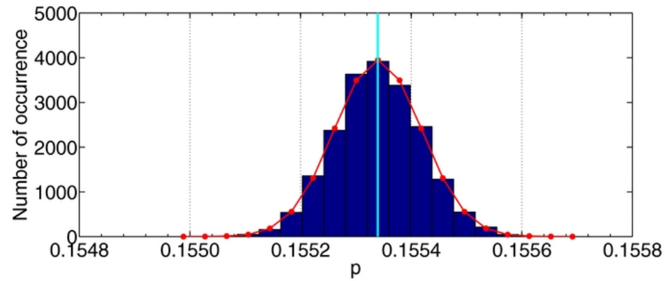
Figure 7. from A New Look at Spitzer Primary Transit Observations of the Exoplanet HD 189733b Morello et al. 2014 ApJ 786 22 doi:10.1088/0004-637X/786/1/22 https://dx.doi.org/10.1088/0004-637X/786/1/22
