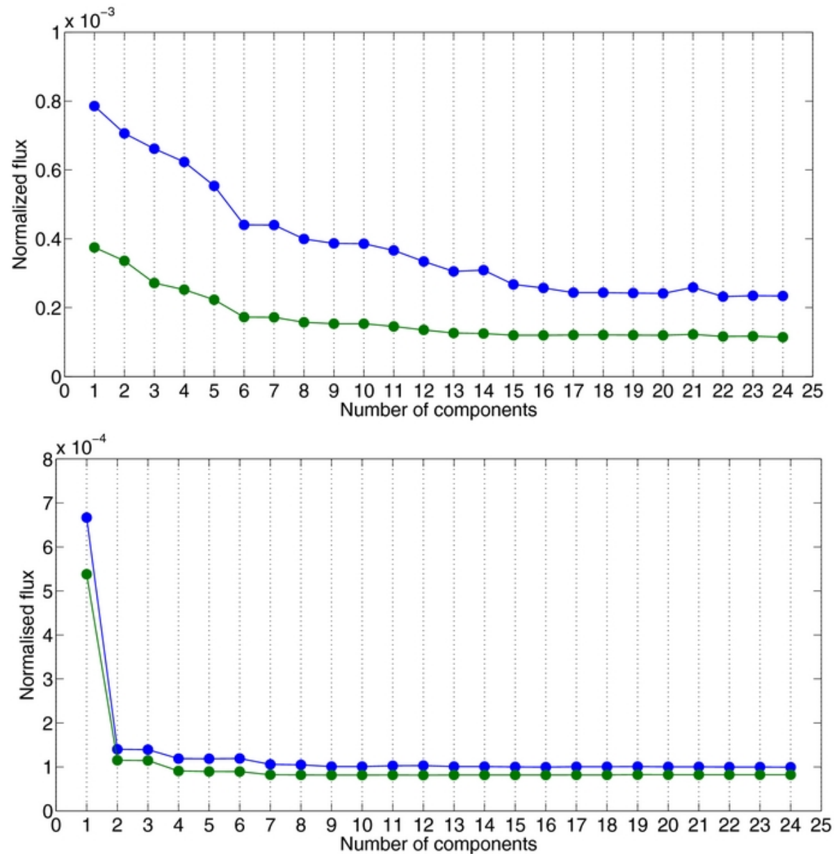
Figure 18. from A New Look at Spitzer Primary Transit Observations of the Exoplanet HD 189733b Morello et al. 2014 ApJ 786 22 doi:10.1088/0004-637X/786/1/22 https://dx.doi.org/10.1088/0004-637X/786/1/22 © 2014. The American Astronomical Society. All rights reserved.
