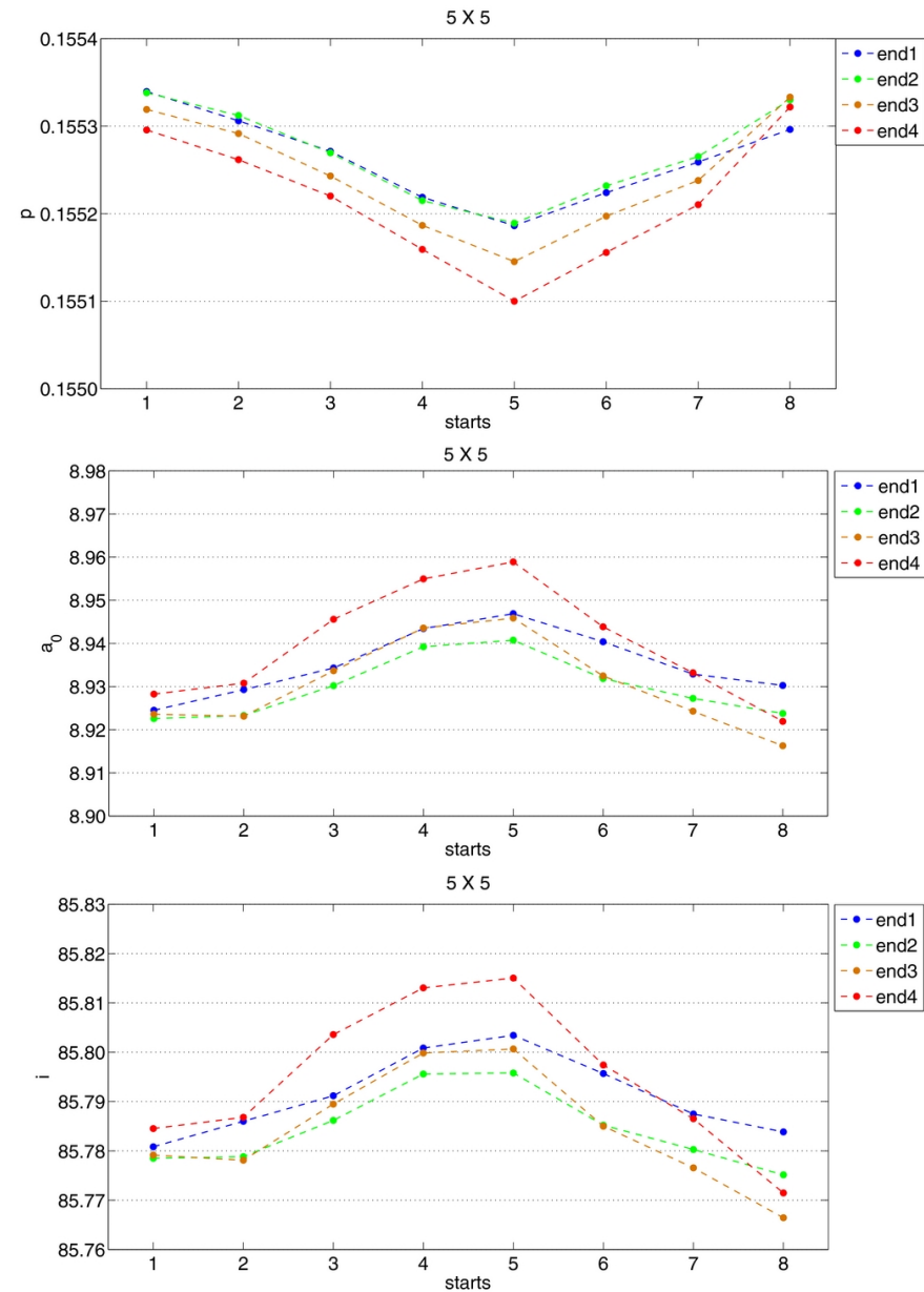
Figure 17. from A New Look at Spitzer Primary Transit Observations of the Exoplanet HD 189733b Morello et al. 2014 ApJ 786 22 doi:10.1088/0004-637X/786/1/22 https://dx.doi.org/10.1088/0004-637X/786/1/22 © 2014. The American Astronomical Society. All rights reserved.
