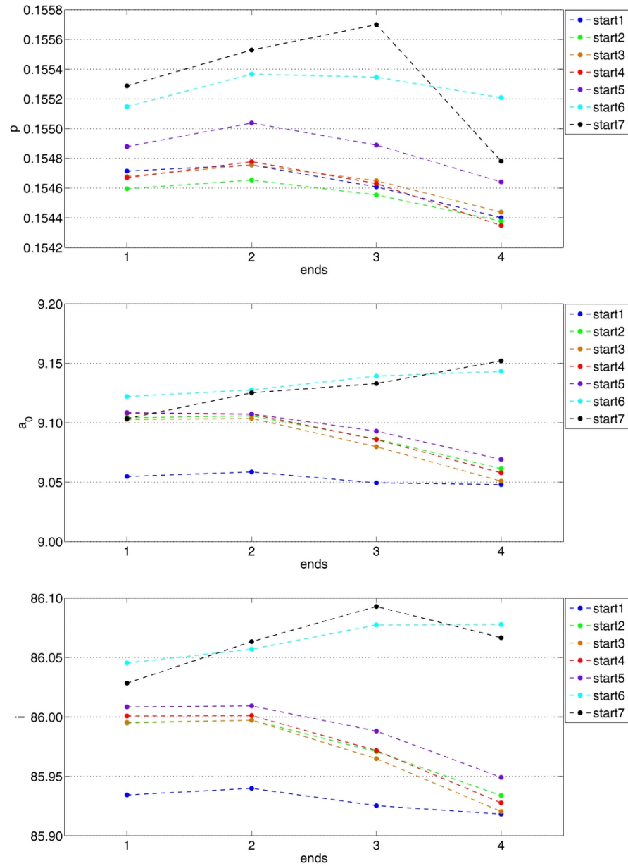
Figure 15. from A New Look at Spitzer Primary Transit Observations of the Exoplanet HD 189733b Morello et al. 2014 ApJ 786 22 doi:10.1088/0004-637X/786/1/22 https://dx.doi.org/10.1088/0004-637X/786/1/22
