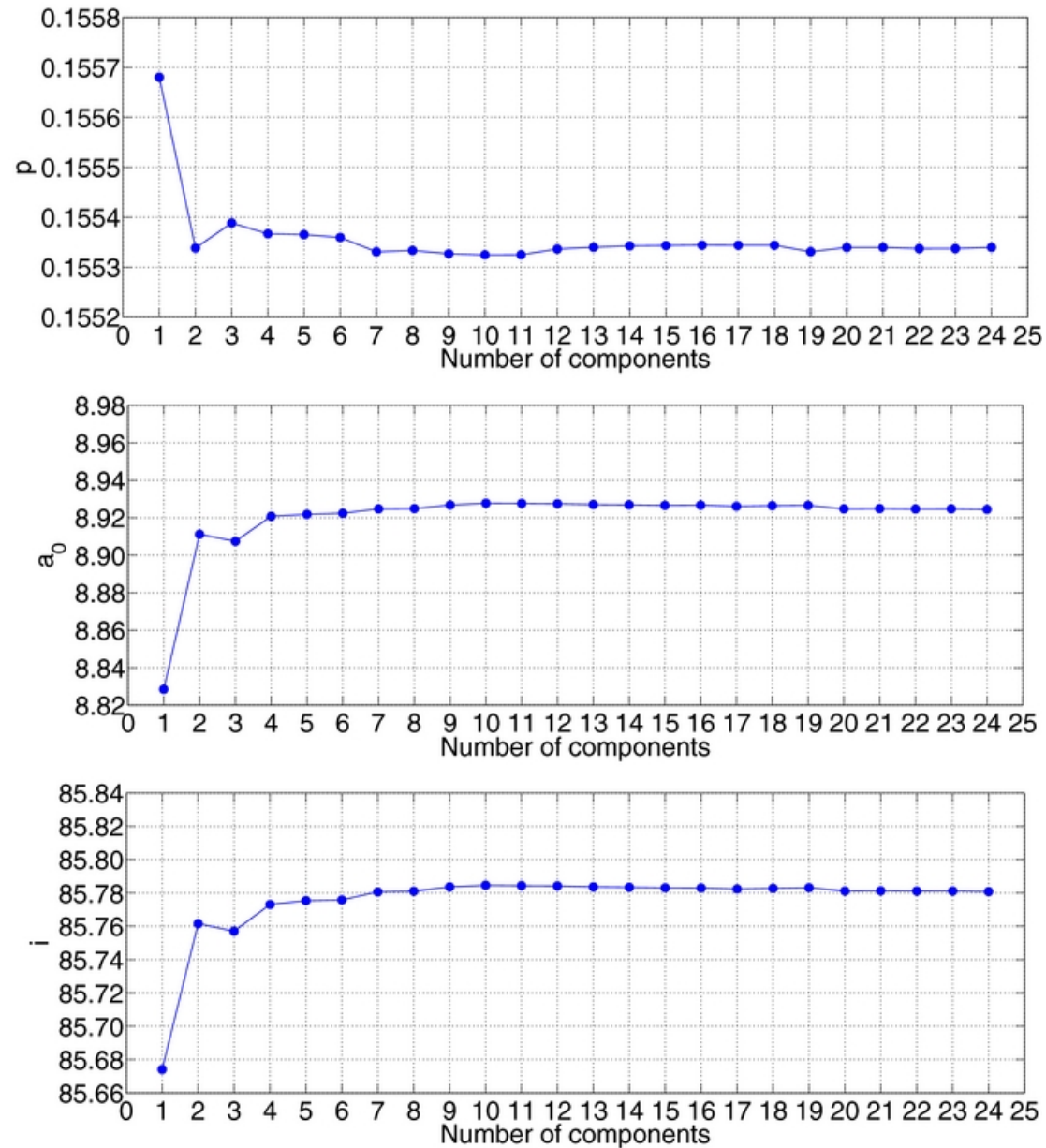
Figure 13. from A New Look at Spitzer Primary Transit Observations of the Exoplanet HD 189733b Morello et al. 2014 ApJ 786 22 doi:10.1088/0004-637X/786/1/22 https://dx.doi.org/10.1088/0004-637X/786/1/22 © 2014. The American Astronomical Society. All rights reserved.
