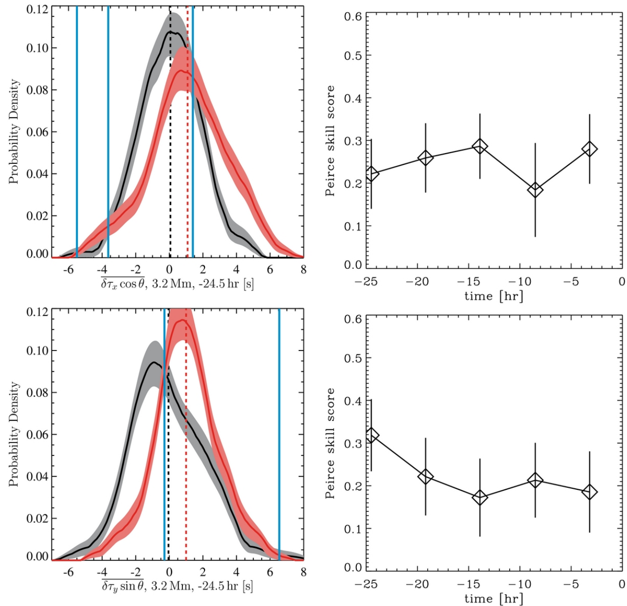
Figure 5. from Helioseismology of Pre-emerging Active Regions. III. Statistical Analysis Barnes et al. 2014 ApJ 786 19 doi:10.1088/0004-637X/786/1/19 https://dx.doi.org/10.1088/0004-637X/786/1/19 © 2014. The American Astronomical Society. All rights reserved.
