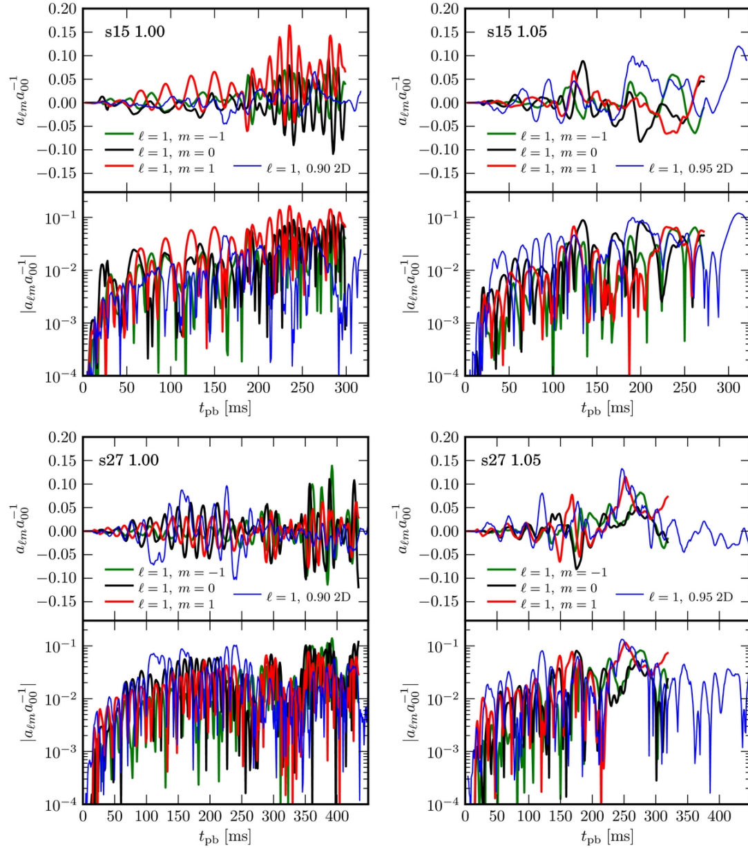
Figure 6. from High-resolution Three-dimensional Simulations of Core-collapse Supernovae in Multiple Progenitors Couch & O'Connor 2014 ApJ 785 123 doi:10.1088/0004-637X/785/2/123 https://dx.doi.org/10.1088/0004-637X/785/2/123
