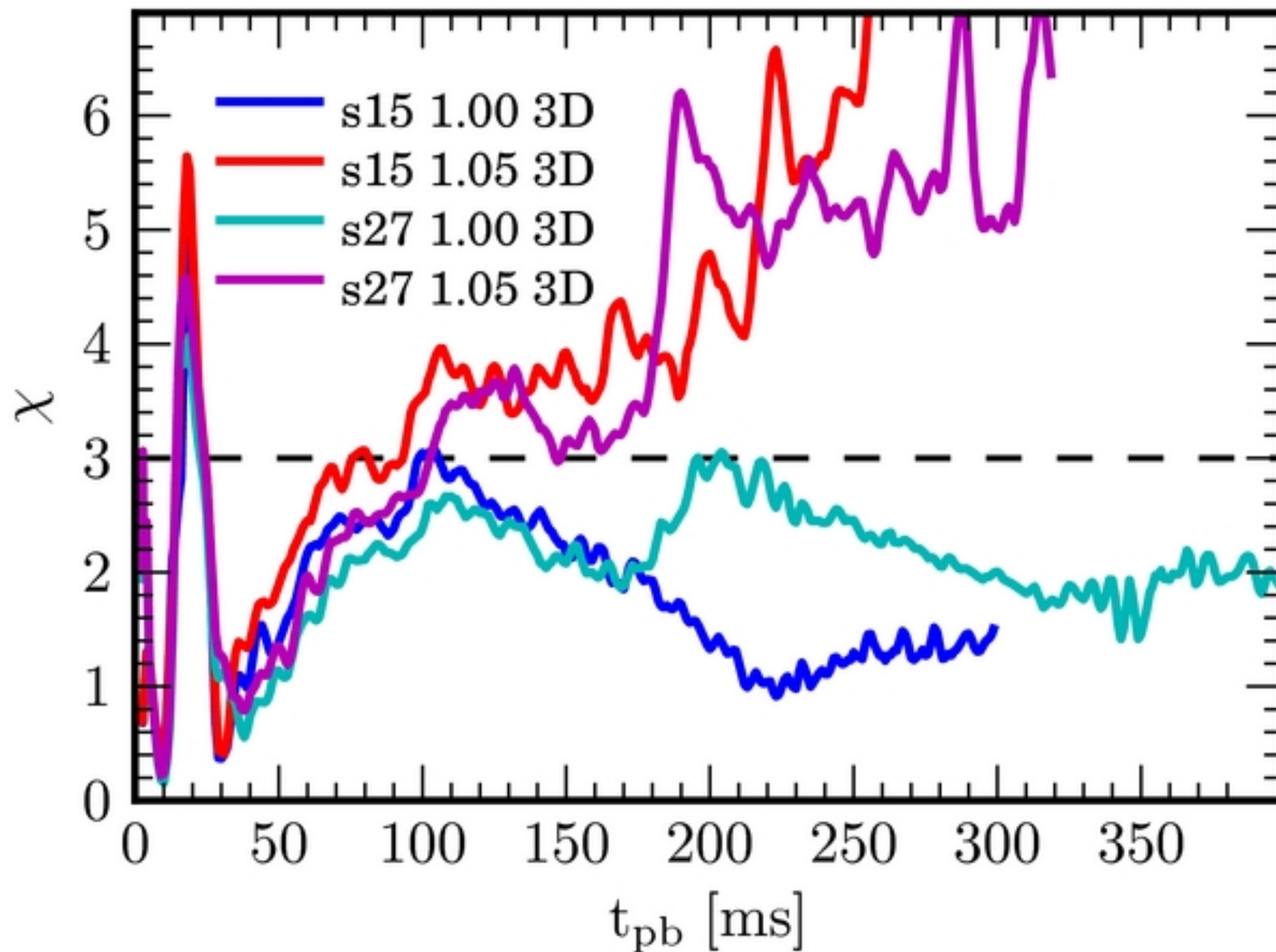
Figure 12. from High-resolution Three-dimensional Simulations of Core-collapse Supernovae in Multiple Progenitors Couch & O'Connor 2014 ApJ 785 123 doi:10.1088/0004-637X/785/2/123 https://dx.doi.org/10.1088/0004-637X/785/2/123 © 2014. The American Astronomical Society. All rights reserved.
