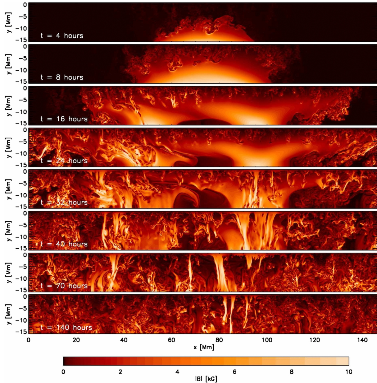
Figure 3. from Numerical Simulations of Active Region Scale Flux Emergence: From Spot Formation to Decay Rempel & Cheung 2014 ApJ 785 90 doi:10.1088/0004-637X/785/2/90 https://dx.doi.org/10.1088/0004-637X/785/2/90
