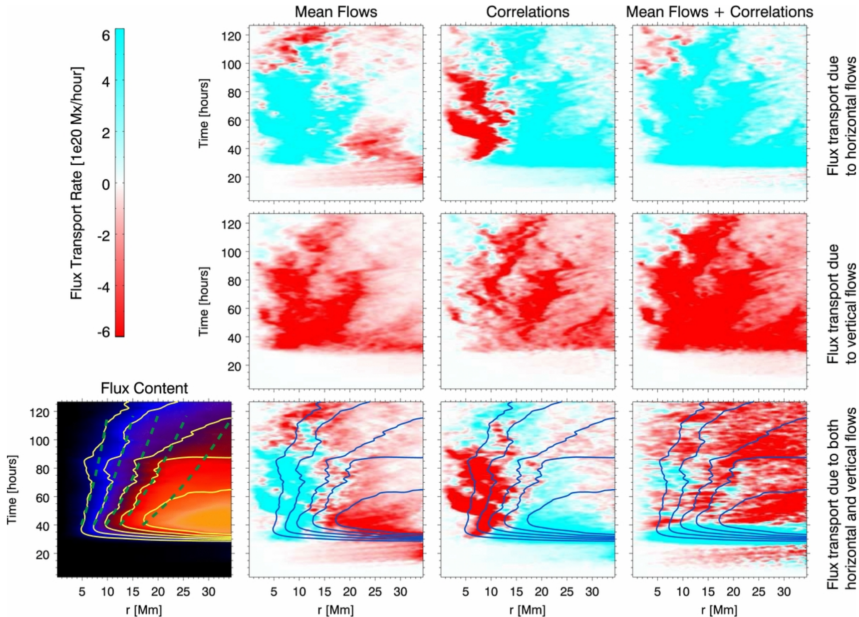
Figure 11. from Numerical Simulations of Active Region Scale Flux Emergence: From Spot Formation to Decay Rempel & Cheung 2014 ApJ 785 90 doi:10.1088/0004-637X/785/2/90 https://dx.doi.org/10.1088/0004-637X/785/2/90
