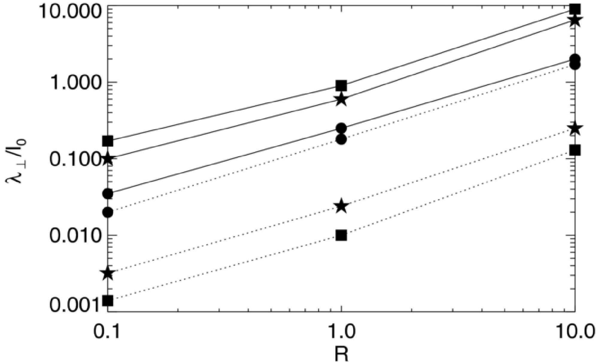
Figure 9. from Detailed Numerical Investigation of the Bohm Limit in Cosmic Ray Diffusion Theory Hussein & Shalchi 2014 ApJ 785 31 doi:10.1088/0004-637X/785/1/31 https://dx.doi.org/10.1088/0004-637X/785/1/31 © 2014. The American Astronomical Society. All rights reserved.
