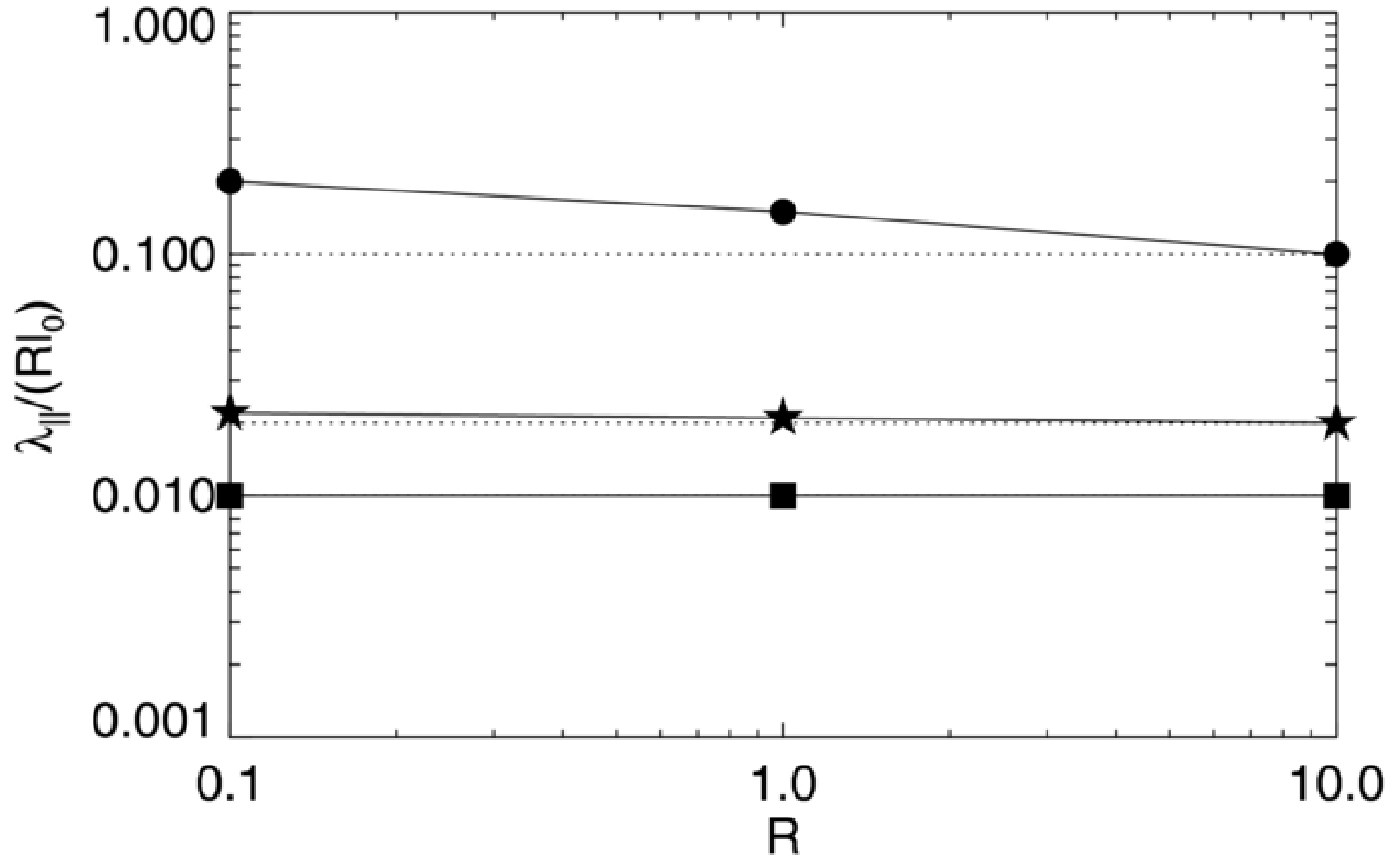
Figure 7. from Detailed Numerical Investigation of the Bohm Limit in Cosmic Ray Diffusion Theory Hussein & Shalchi 2014 ApJ 785 31 doi:10.1088/0004-637X/785/1/31 https://dx.doi.org/10.1088/0004-637X/785/1/31 © 2014. The American Astronomical Society. All rights reserved.
